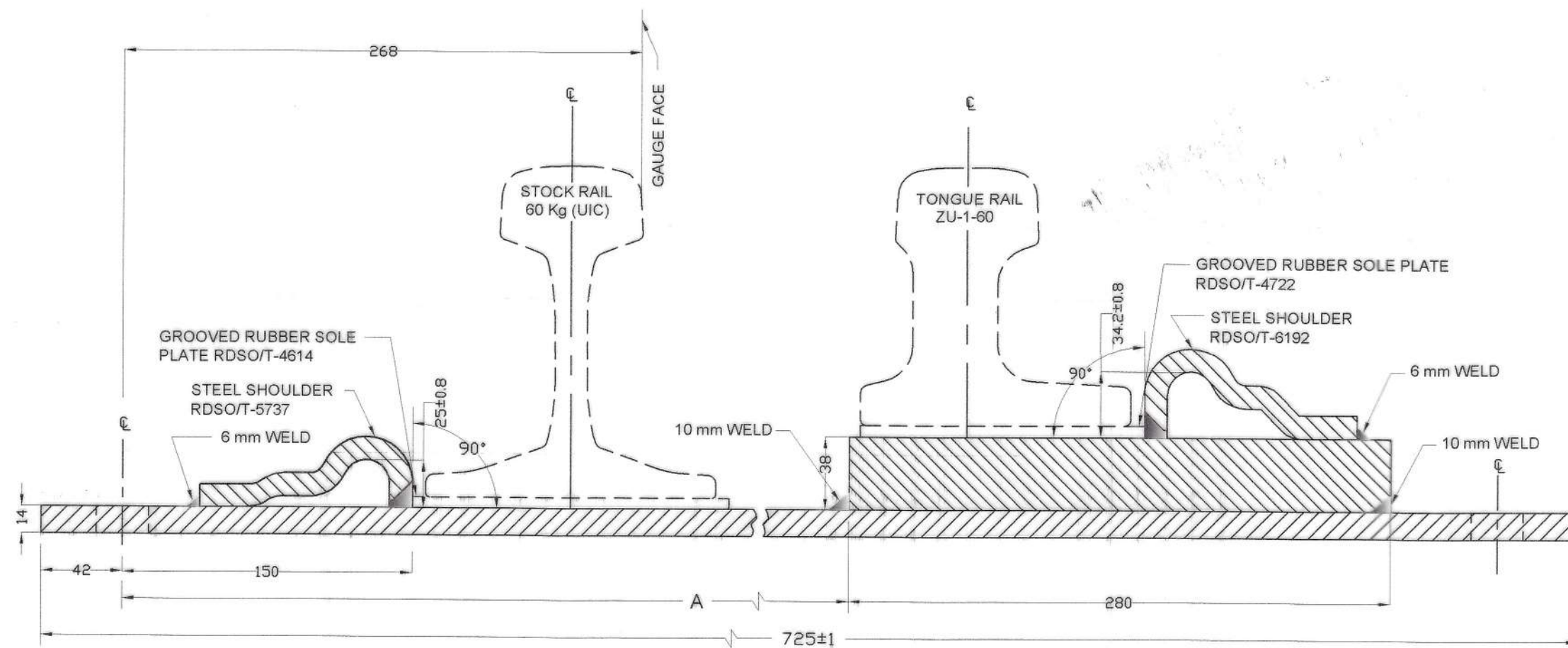
SECTIONAL ELEVATION ON 'AB'
